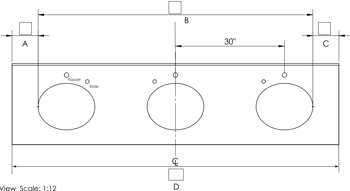
DSCT Plan View Scale: 1:12
